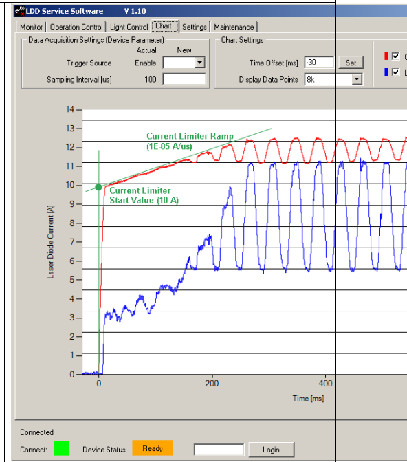
LPC Soft-Start Limitation (green)
