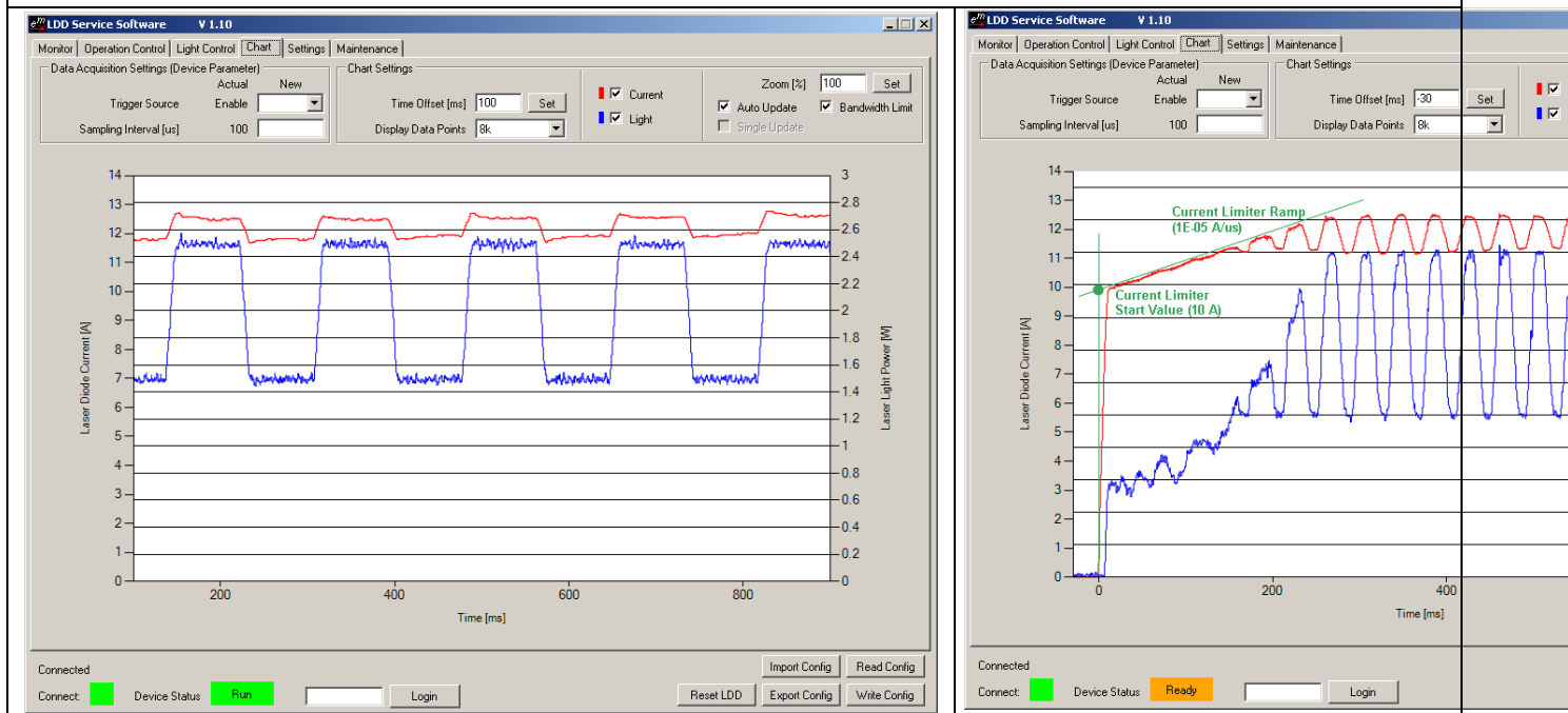
Laser Power Control (blue) and Diode Current (red).
